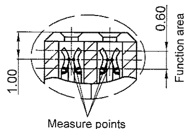
DETAIL Z SCALE 4:1
