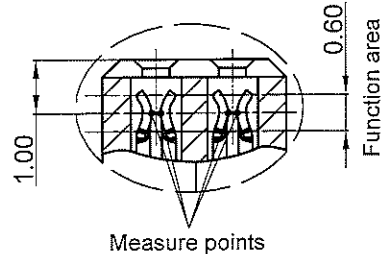
DETAIL Z SCALE 4:1
